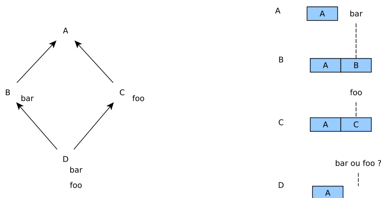
FIGURE 2.4 – Situation d’héritage multiple
